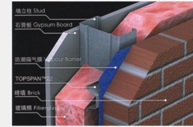
Exterior Wall Type 3 外墙类型3
