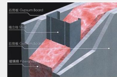
Exterior Wall Type 7 外墙类型7
