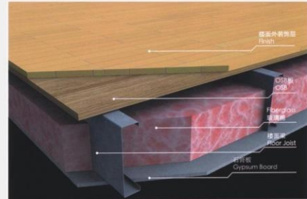
Floor Type 3 楼面类型3
