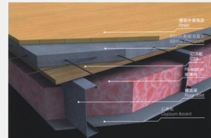
Floor Type 2 楼面类型2
